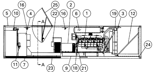
3516 4-Turbo Power Module Interior Layout Roadside View
